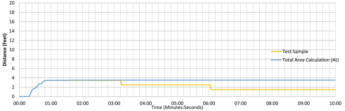
Smoke Readings
